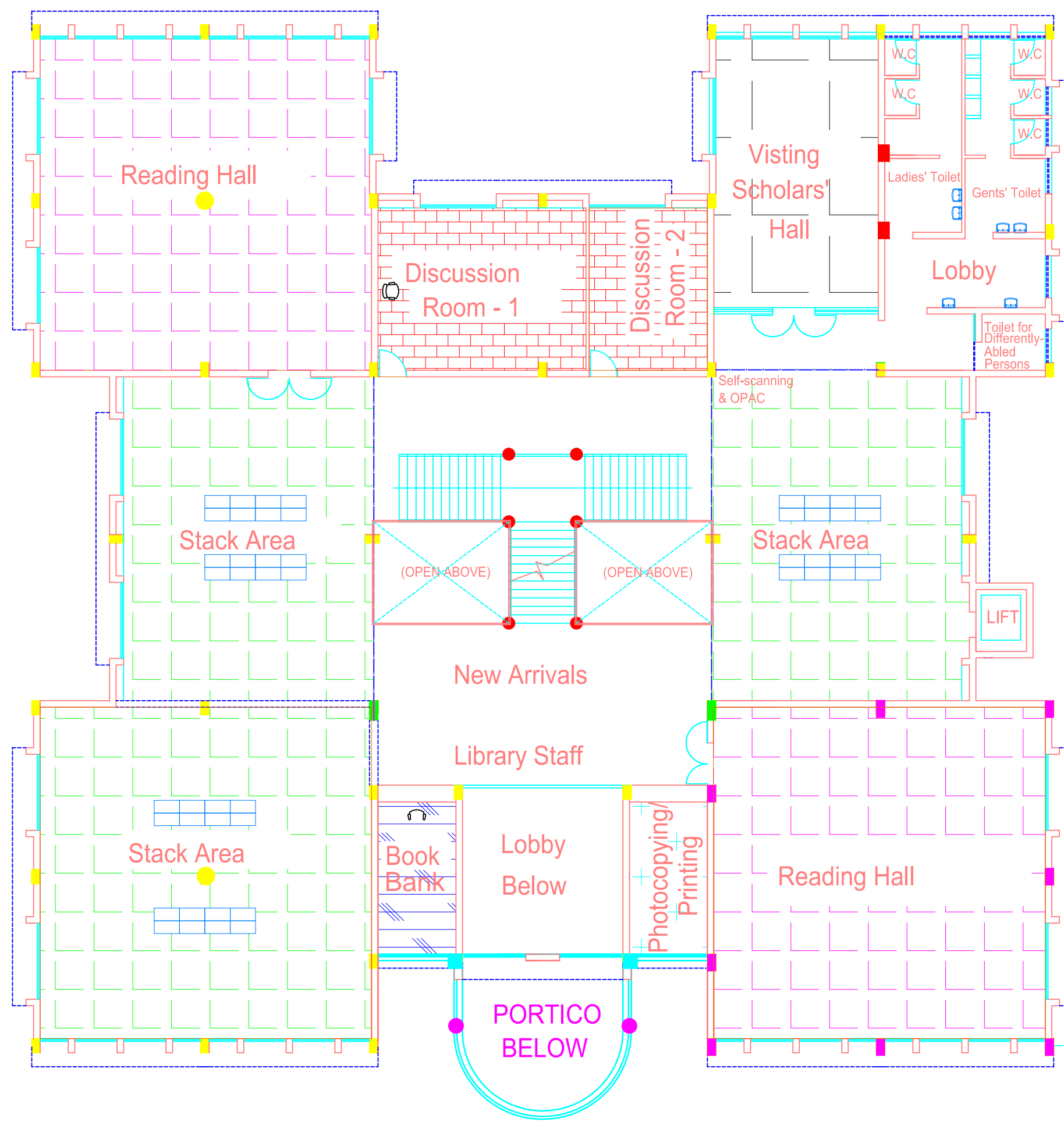
FIRST FLOOR AREA: 1136 sq.mts.
